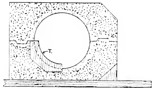
NO. 151. — REVERSE CASTING MOLD FOR PLAIN COLUMNS, SHOWING RUN JOGGLES.
